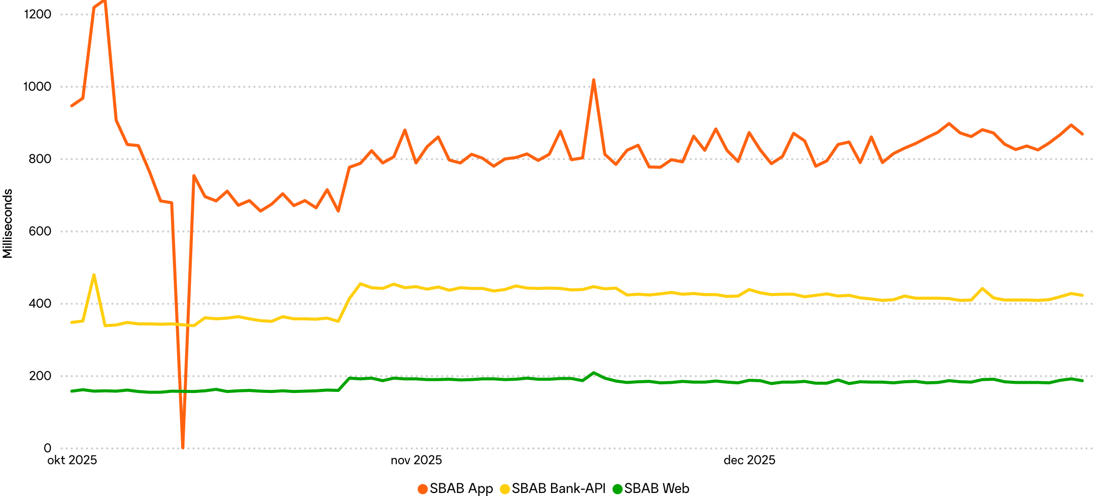
Daily average time to provide account initiation
